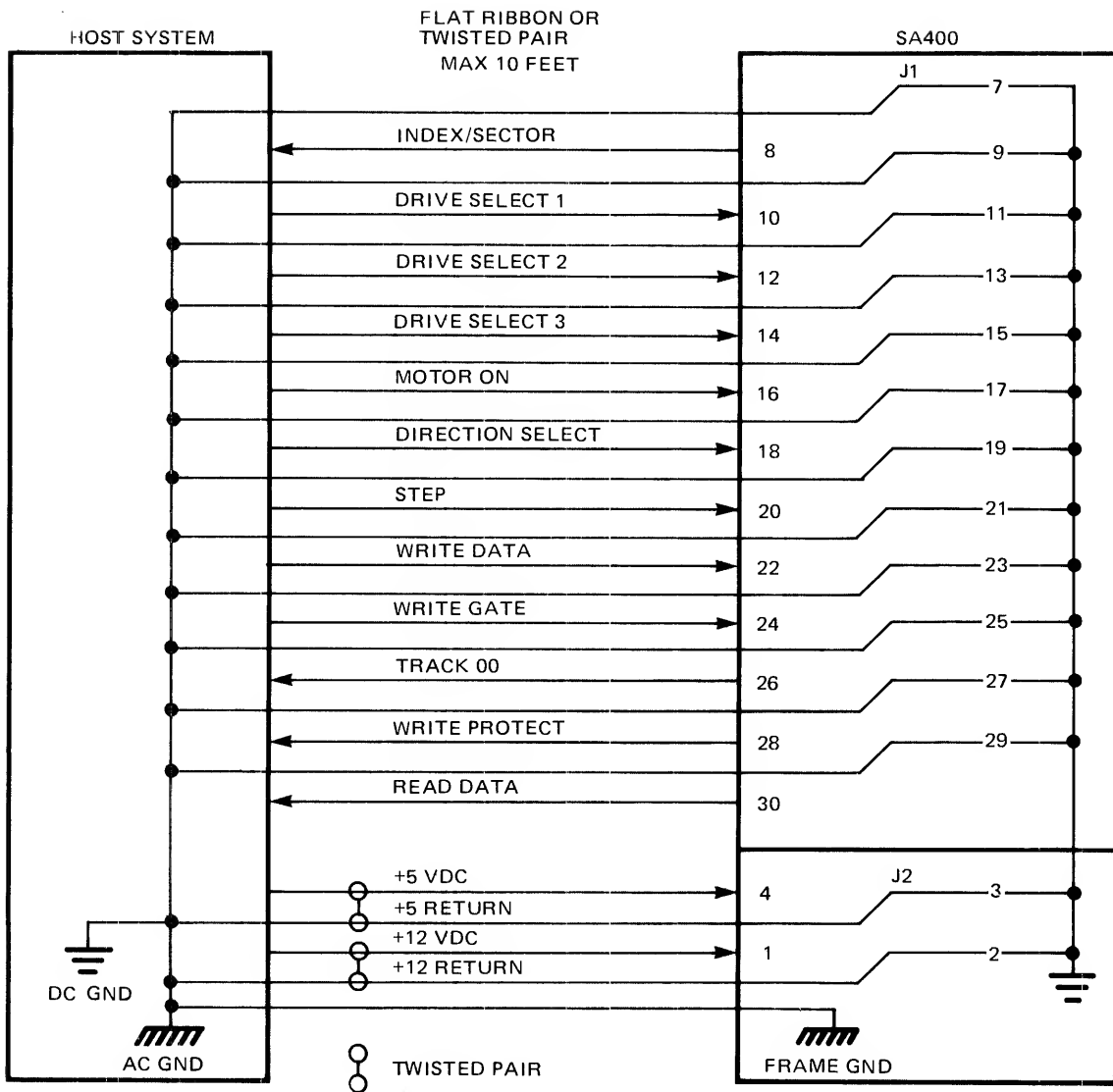
FIGURE 9. INTERFACE CONNECTIONS
